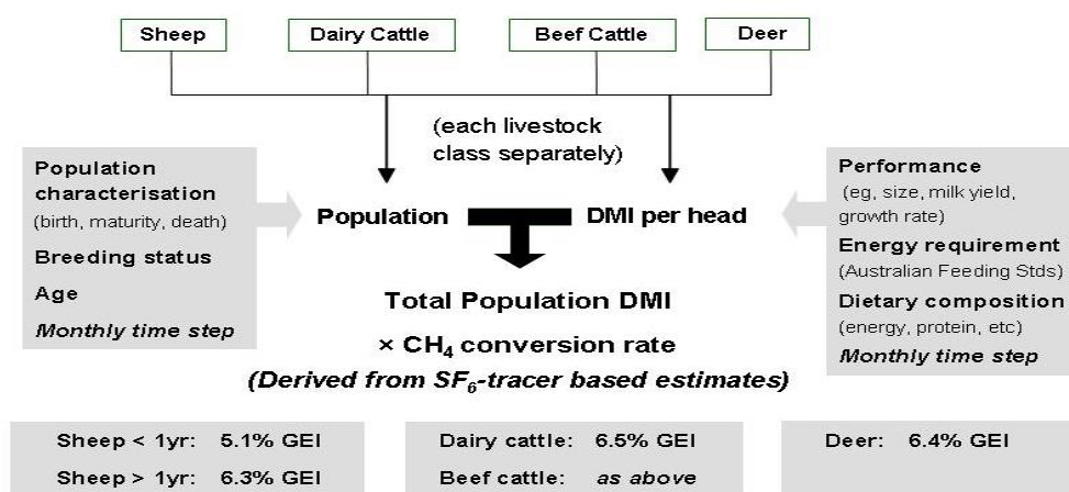
Figure 5.2.1 Schematic diagram of how New Zealand's emissions from enteric fermentation are calculated
