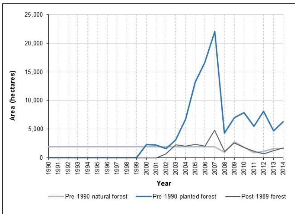
Figure 11.3.1 New Zealand's annual areas of deforestation from 1990 to 2014
