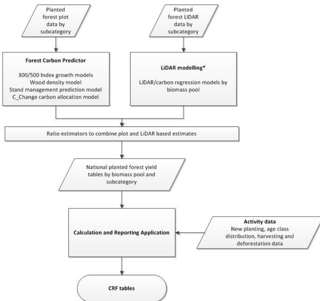
Figure 6.4.6 New Zealand's planted forest inventory modelling process
