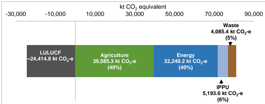
Figure ES 4.2 New Zealand’s gross emissions by sector in 2014
